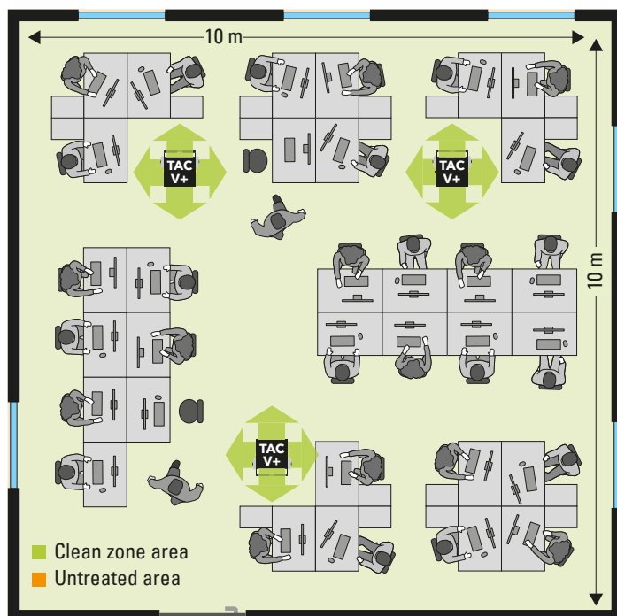
Example of occupancy in a call center: With an area of 10 x 10 m at a room height of 2.5 m, the office zone shown has an air volume of 250 m 3 , which 3 TAC V+ can circulate 19 times per hour (air capacity 4,800 m 3 /h), which corresponds to an air exchange rate (LW/h) of 19 (clean air volume of 150 m 3 per person with 32 occupied workplaces) – almost a factor of 8 compared to the aircraft!
